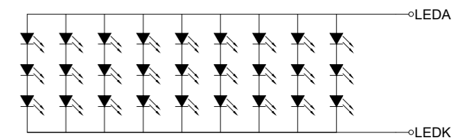
LED Diagram Circuit
